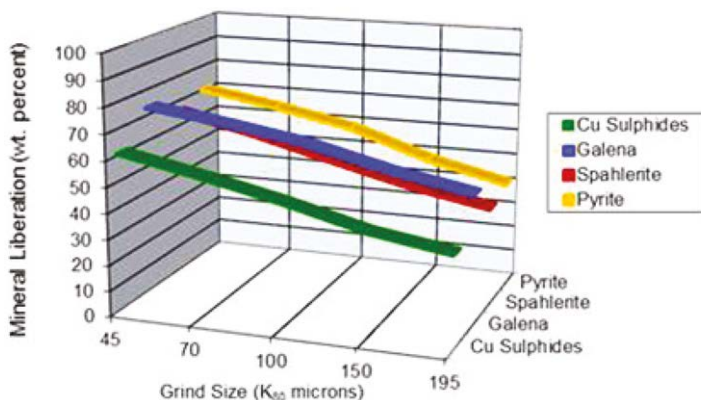
Effect of Primary Grind on Mineral Liberation
